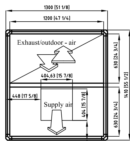
Section B
