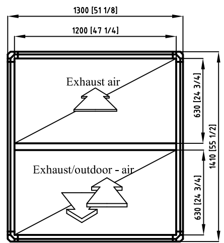
Section A
